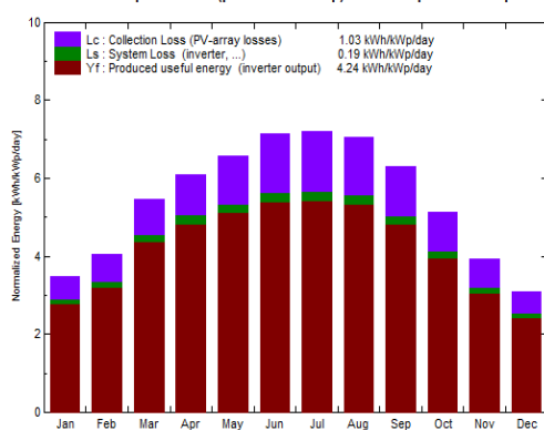
Normalized productions (per installed kWp): Nominal power 25 kWp
