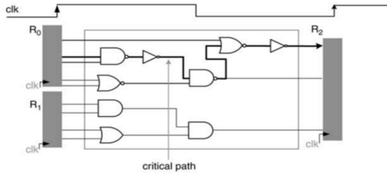
12: Critical Path
