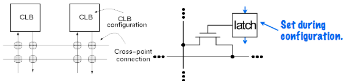
20: Interconnection Detail
