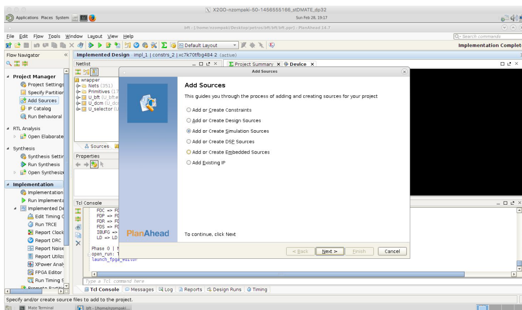
53: Add simulation sources
