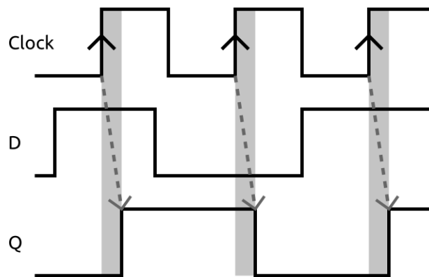
15: Propagation Time
