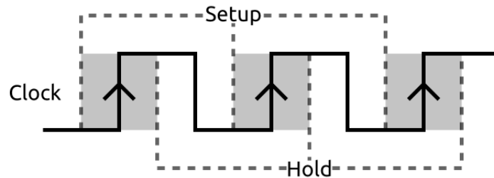
14: Setup and Hold Time
