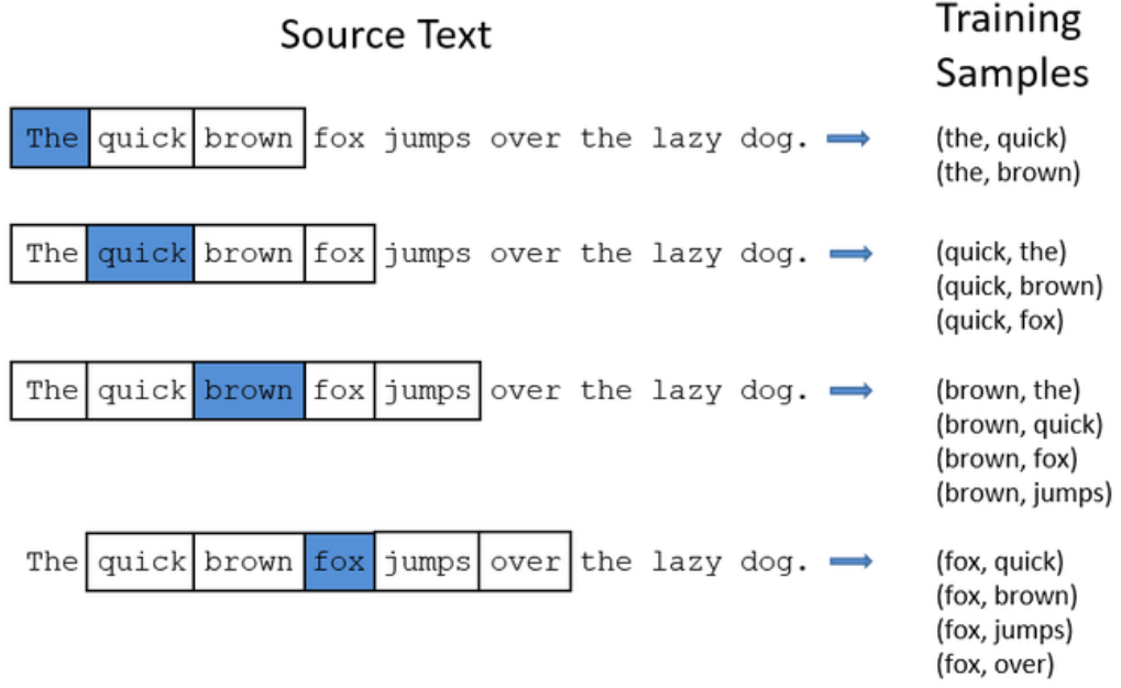
Figure 3.5: Example of Word2vec's processing on a sentence
