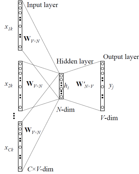
Figure 3.6: CBOW's architecture
