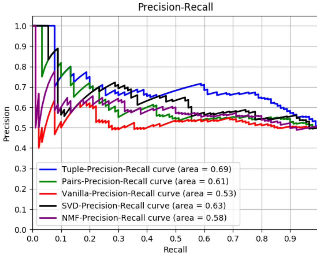
Figure 5.2: Precision-Recall: Our testing results
