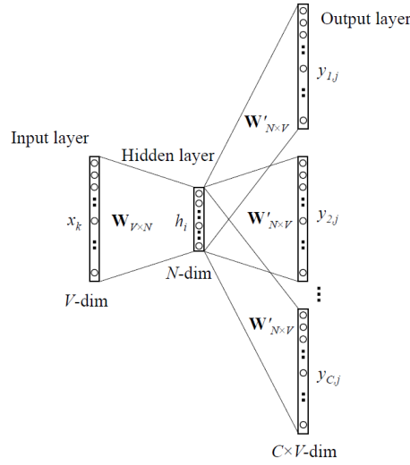
Figure 3.8: Skip-gram's architecture
