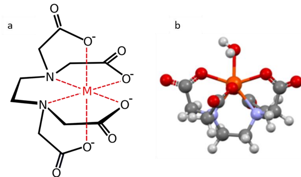
Fig. 5: (a) The metal-EDTA chelate as found in the Co (III) complexes; and (b) The structure of [Fe (EDTA) (H 2 O)] - , indicating that the EDTA 4 ligand does not completely encapsulate Fe (III), which is seven-coordinated
