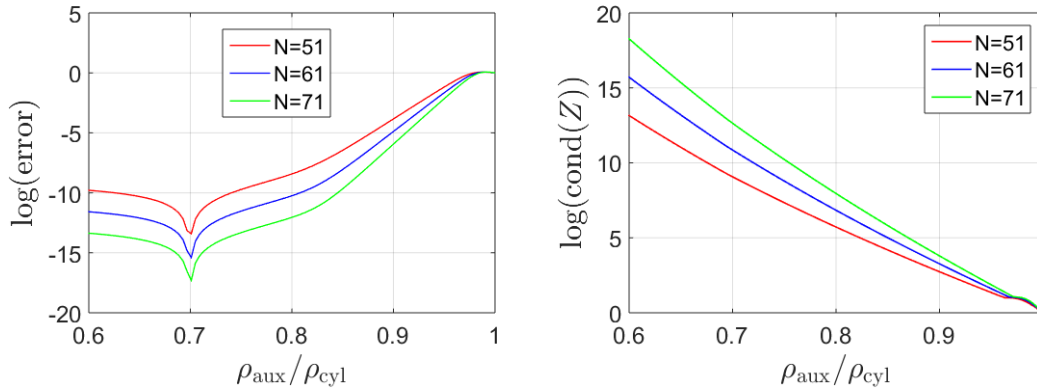
FIGURE 2.6: Boundary condition error (left panel) and matrix condition number (right panel) versus \rho_{\text{aux}} / \rho_{\text{cyl}} for the application of MAS to the circular cylinder (cf. Figs. 2.4 and 2.5) with N = 51, 61, 71 .
