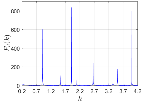
FIGURE 3.5: As in Fig. 3.4, but for TE modes and using an internal line source without a regularization method.
