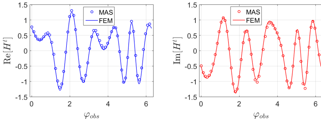
FIGURE 2.13: Real and imaginary parts of the total magnetic field H^t at \sigma_{\text{obs}} = 4 versus \phi_{\text{obs}} . For MAS, the values of the diverging MAS currents of Fig. 2.12 are used.
