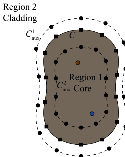
FIGURE 5.10: Application of MAS-TES for a dielectric waveguide with inverted-elliptical core.
