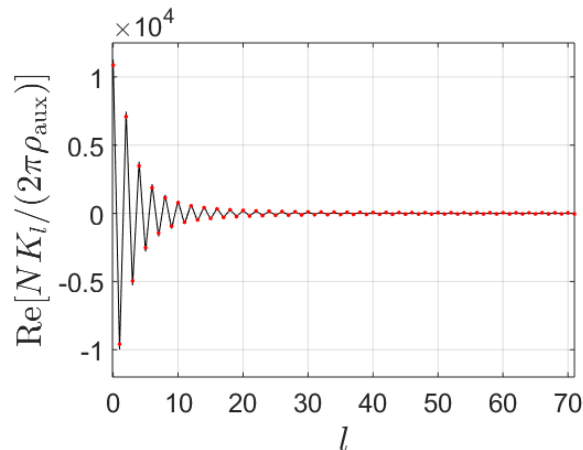
FIGURE 2.8: Real part of the normalized MAS currents NK_l / (2\pi\rho_{\text{aux}}) versus the source index l for k\rho_{\text{aux}} = 1.3 and N = 140 . Red dots correspond to the asymptotic formula (2.27), while black straight lines to the numerical solution of the system (2.14). For clarity, we show only results corresponding to l = 0, 1, \dots, 71 (currents for l > 70 are symmetric with respect to those for l < 70 ).
