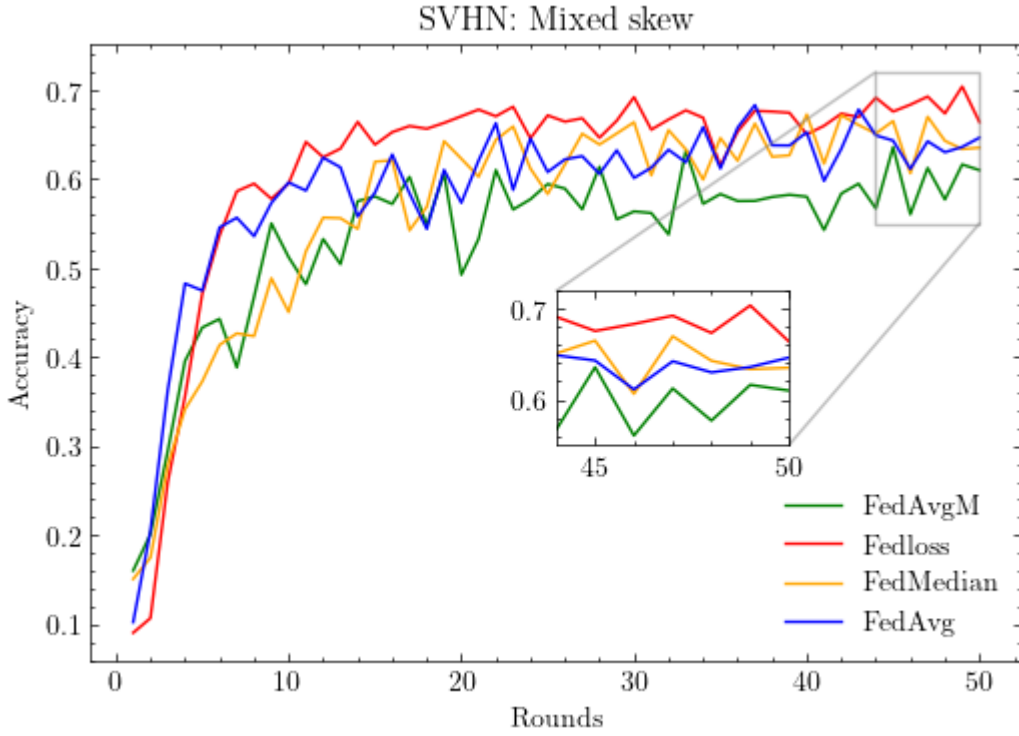
Figure 20: Results for the SVHN task in mixed skew setting.
