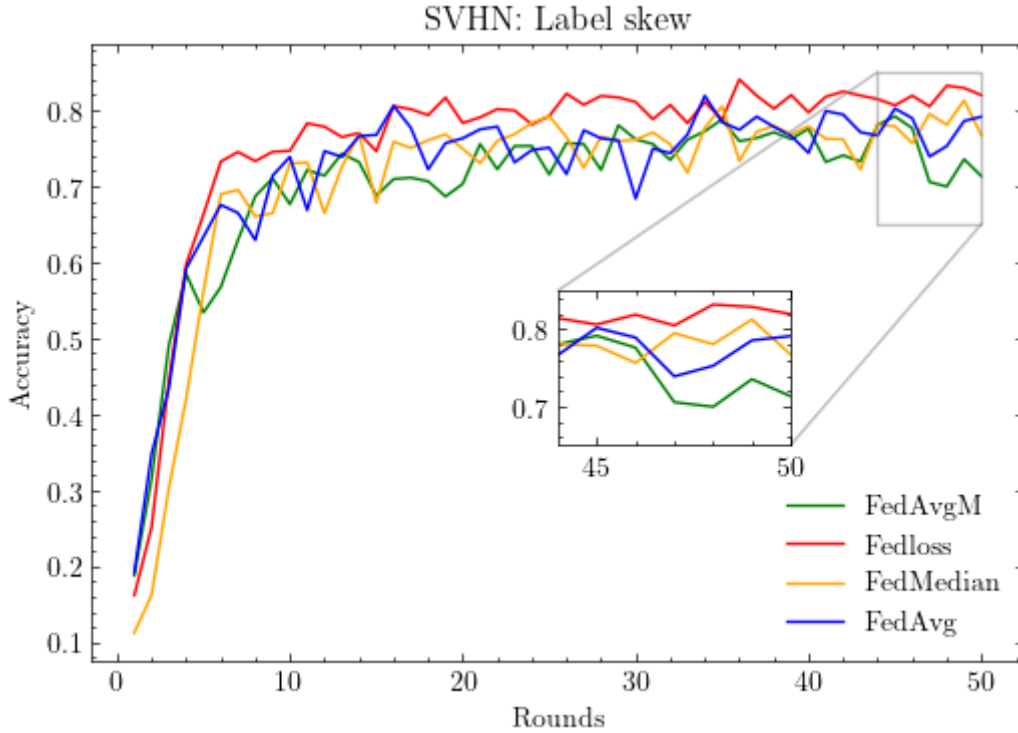
Figure 14: Results for the SVHN task in label skew setting.
