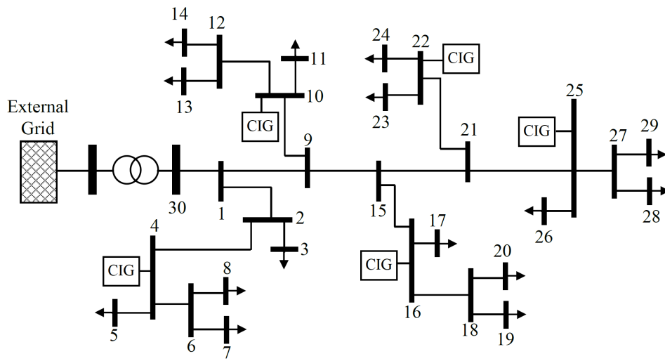
Figure 4.6: 30-bus feeder
