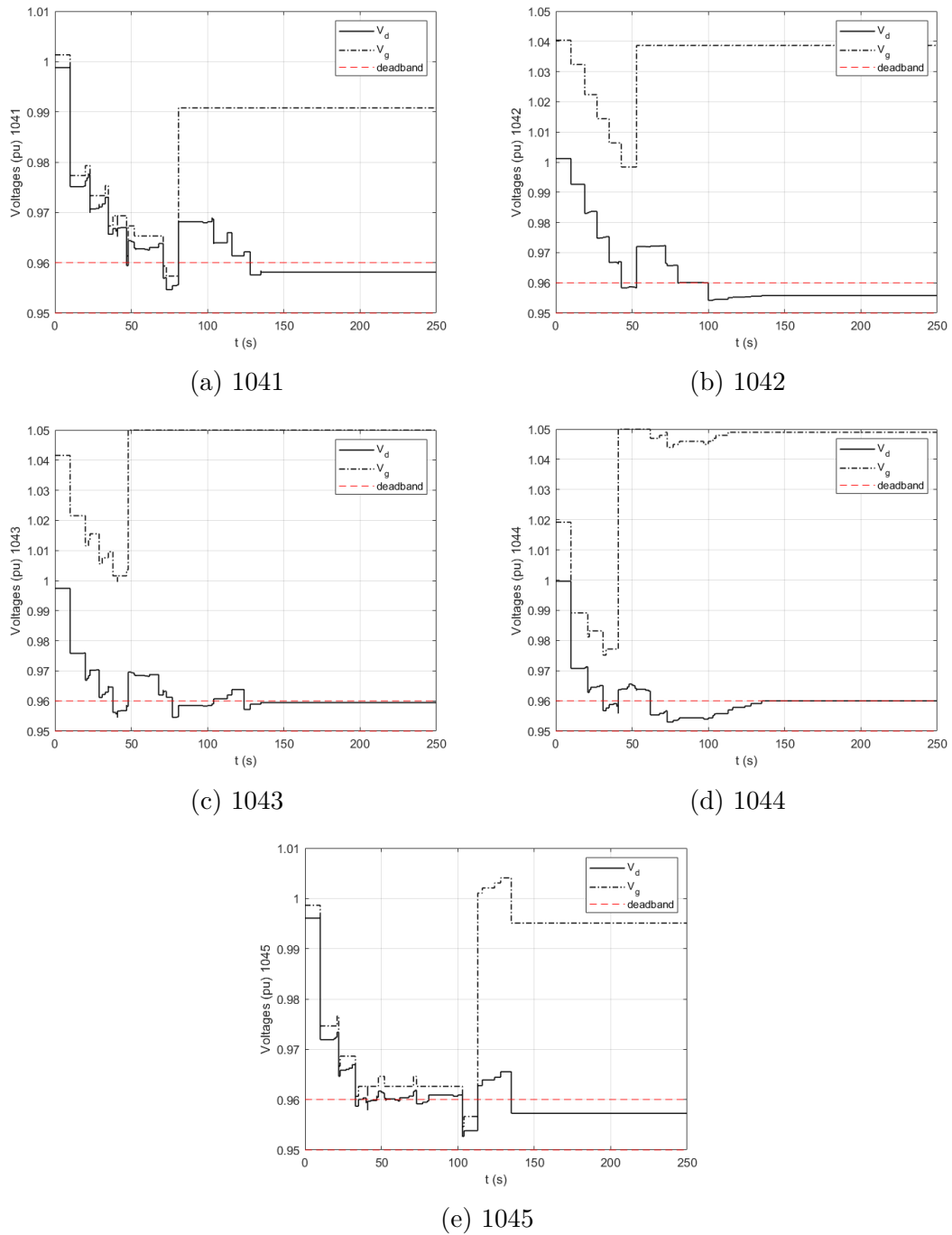
Figure 5.4: Setpoint implementation in ADNs connected in the 5 HV buses
