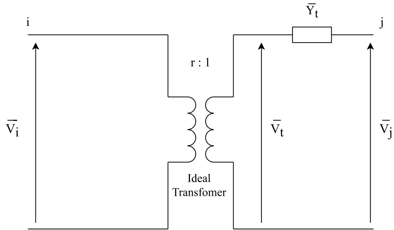
Figure 4.3: Standard equivalent circuit for a transformer
