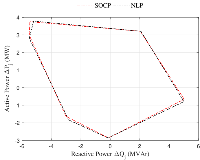
Figure 6.12: FR Polygon approximation of 99-bus, SOCP vs NLP
