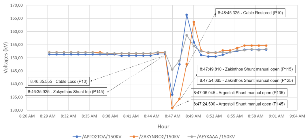
Figure 7.4: Events and voltages in Ionian islands
