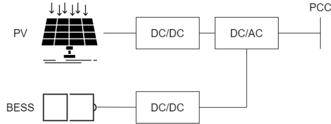
Figure 4.2: Solar panel with BESS
