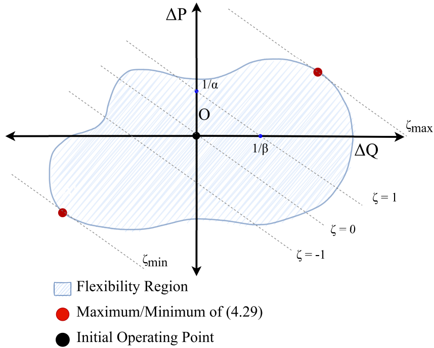
Figure 4.9: Typical FR of an ADN
