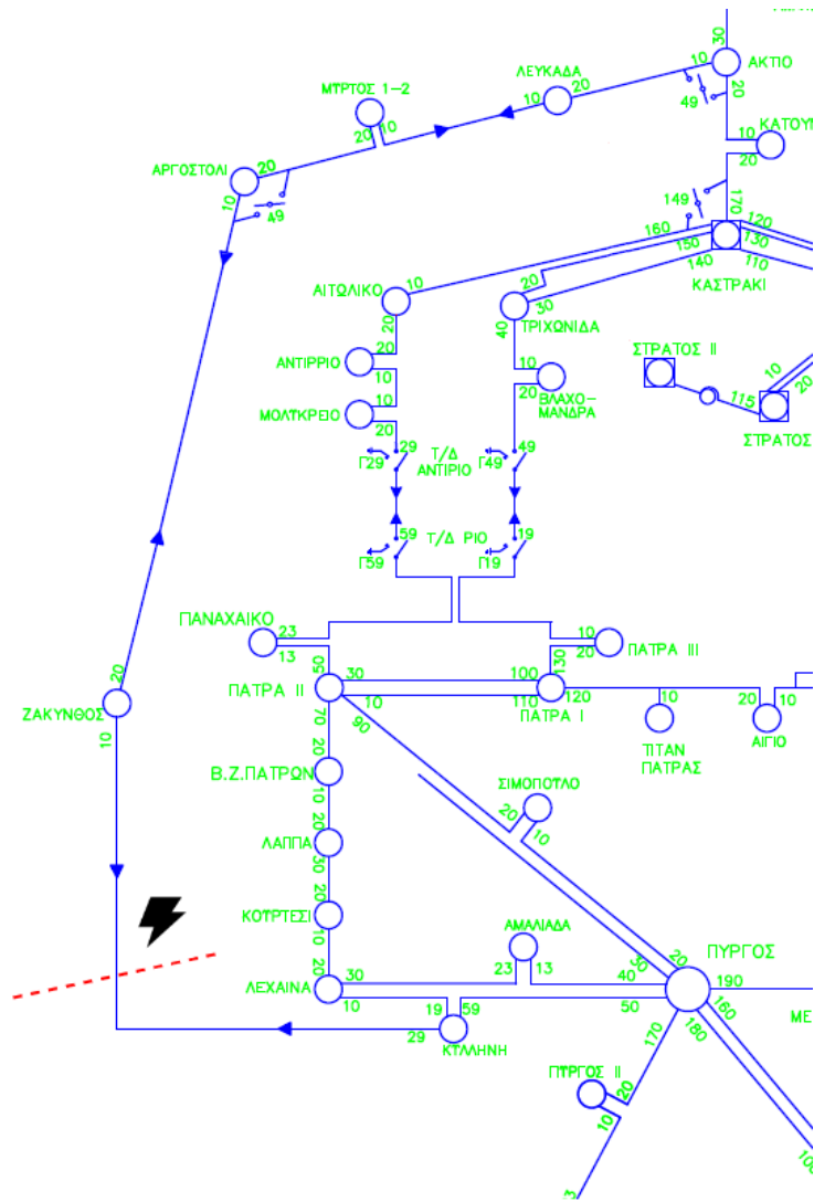
Figure 7.3: Ionian Islands Transmission Corridor
