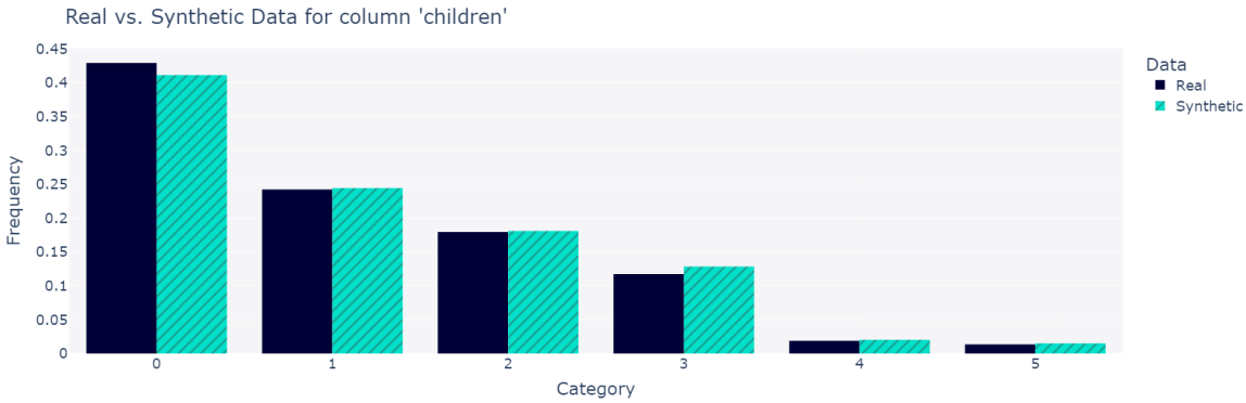
Figure 55: Children distribution
