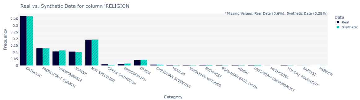
Figure 102: Religion distribution
