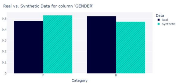
Figure 74: Gender distribution
