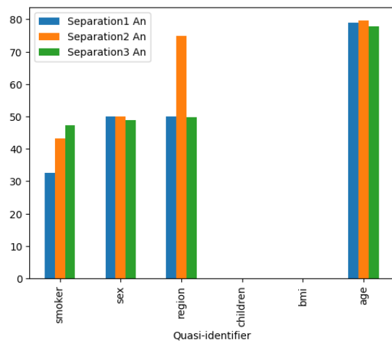
Figure 49: Separation after anonymisation for medical cost
