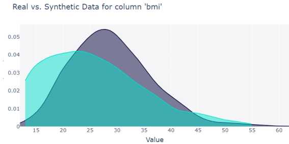
Figure 77: Bmi distribution
