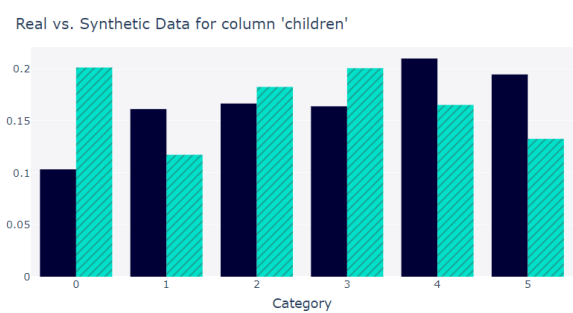
Figure 75: Children distribution
