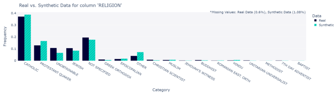
Figure 110: Religion distribution
