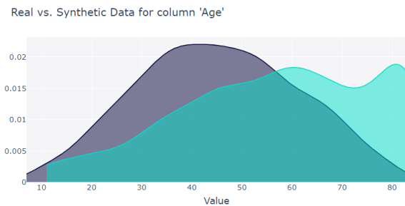
Figure 79: Age distribution
