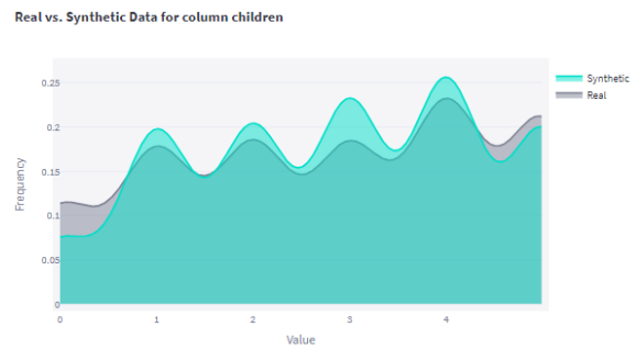
Figure 66: Children distribution
