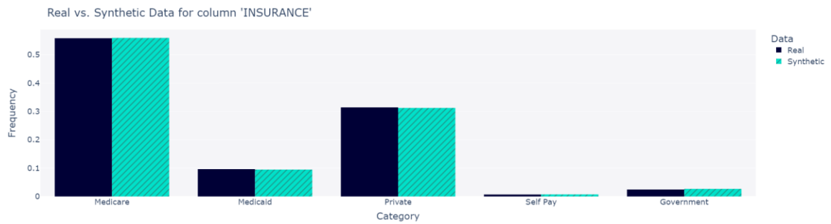
Figure 100: Insurance distribution
