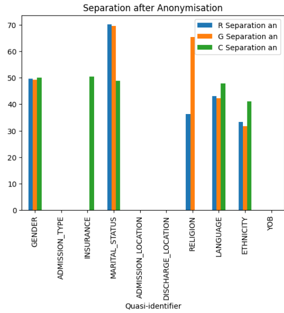
Figure 120: Separation after anonymisation for admissions
