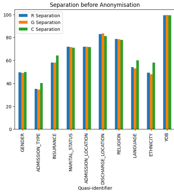
Figure 119: Separation before anonymisation for admissions
