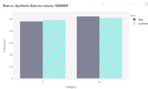
Figure 65: Gender distribution
