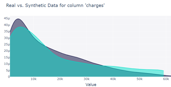
Figure 78: Charges distribution
