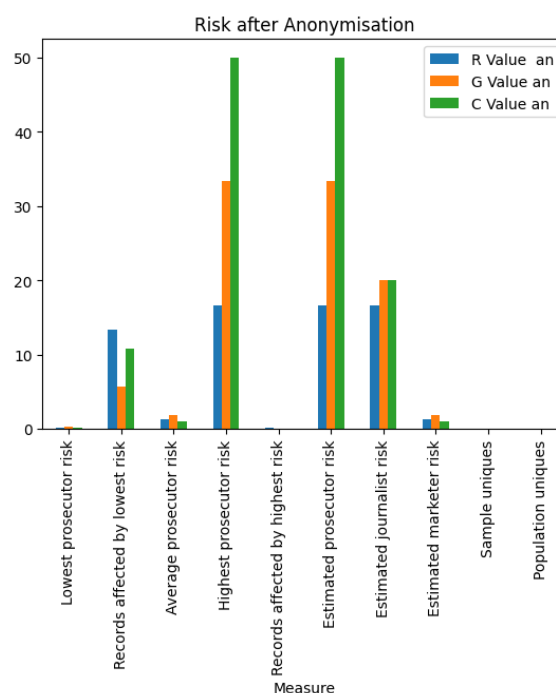
Figure 114: Risk after anonymisation for admissions
