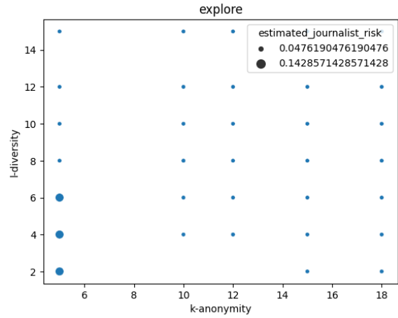
Figure 13: Estimated journalist risk
